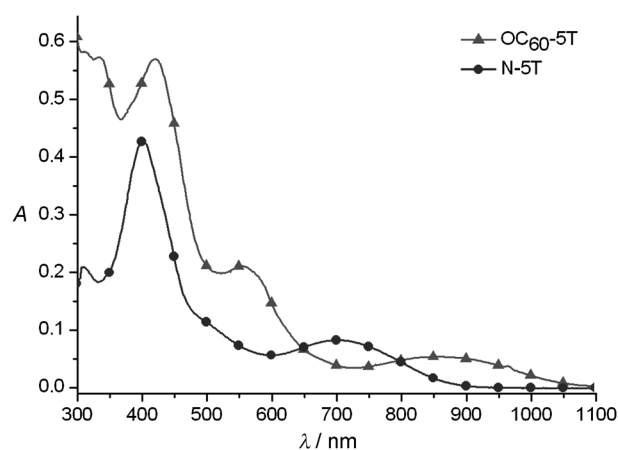
Figure 4. UV/Vis–NIR spectra of OC 60 -5T and N-5T in CHCl 3 ( 10^{-5} \text{ M} ).
